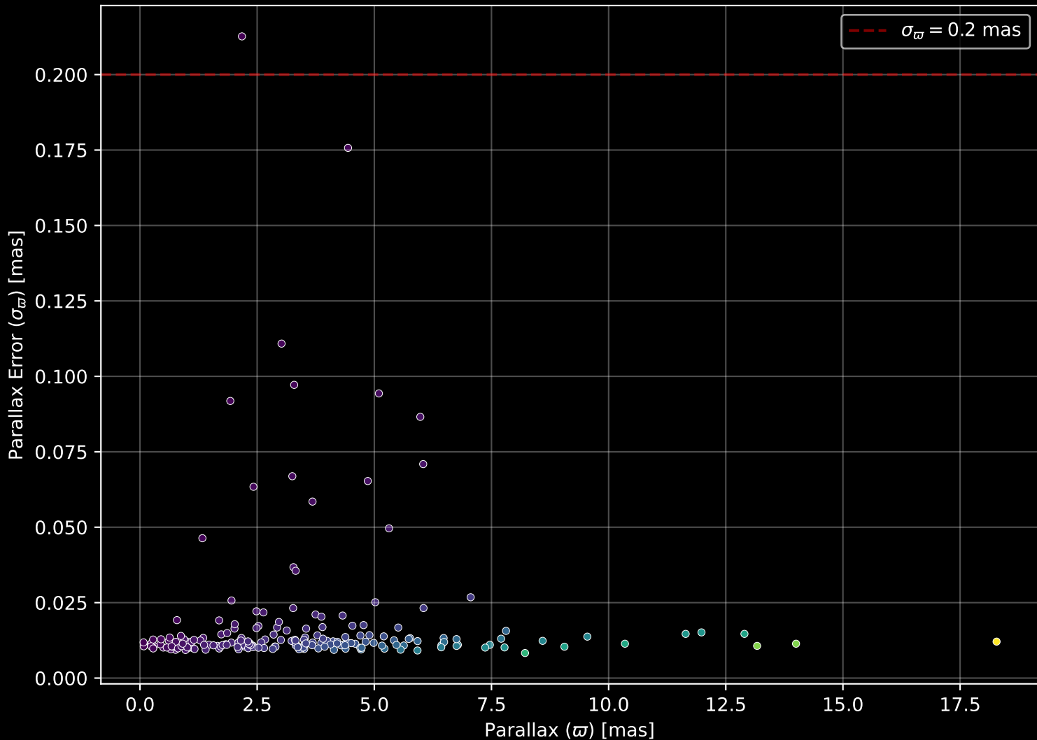
APOGEE DR17 Field: [081+49_MGA] Parallax Quality (n= 195)
