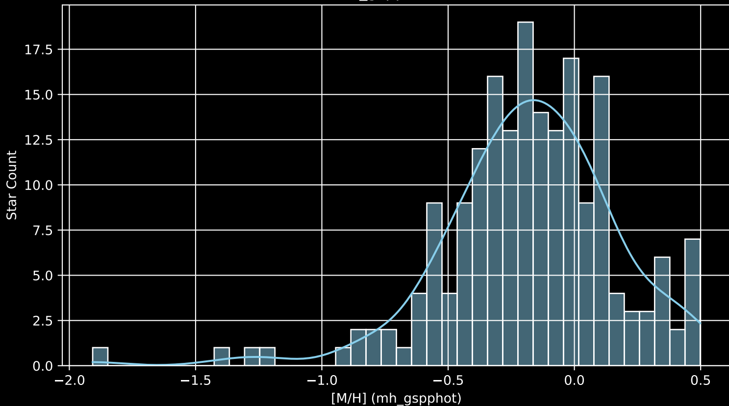
APOGEE DR17 Field: [081+49_MGA [M/H] (mh_gspphot) (n= 192)
