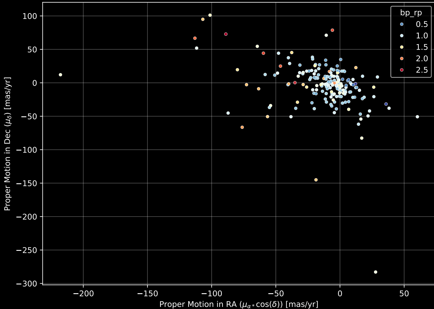
APOGEE DR17 Field: [081+49_MGA] Proper Motion Diagram (n= 195)
