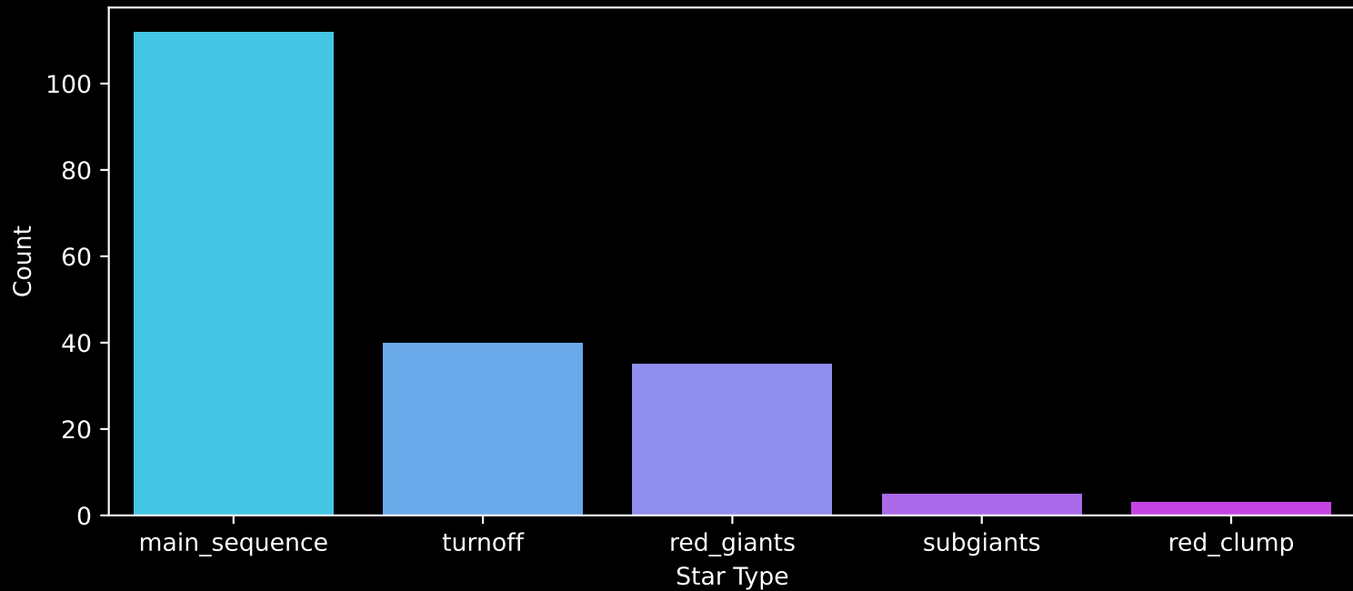
APOGEE DR17 Field: [081+49_MGA] Count plot of Star Type
