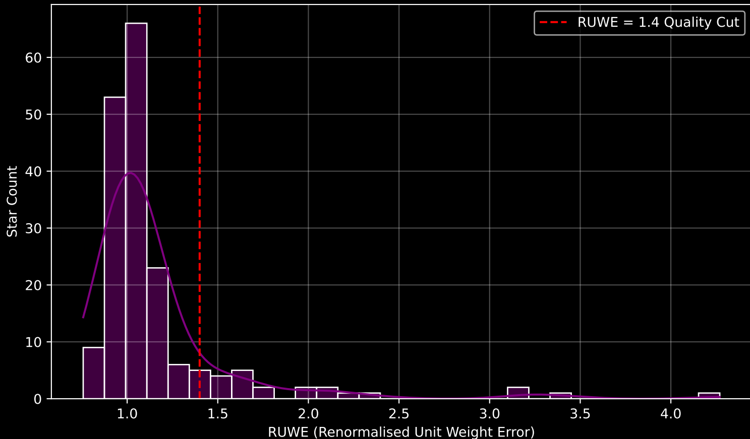
GAPOGEE DR17 Field [081+49_MGA] RUWE Distribution (n= 183)
