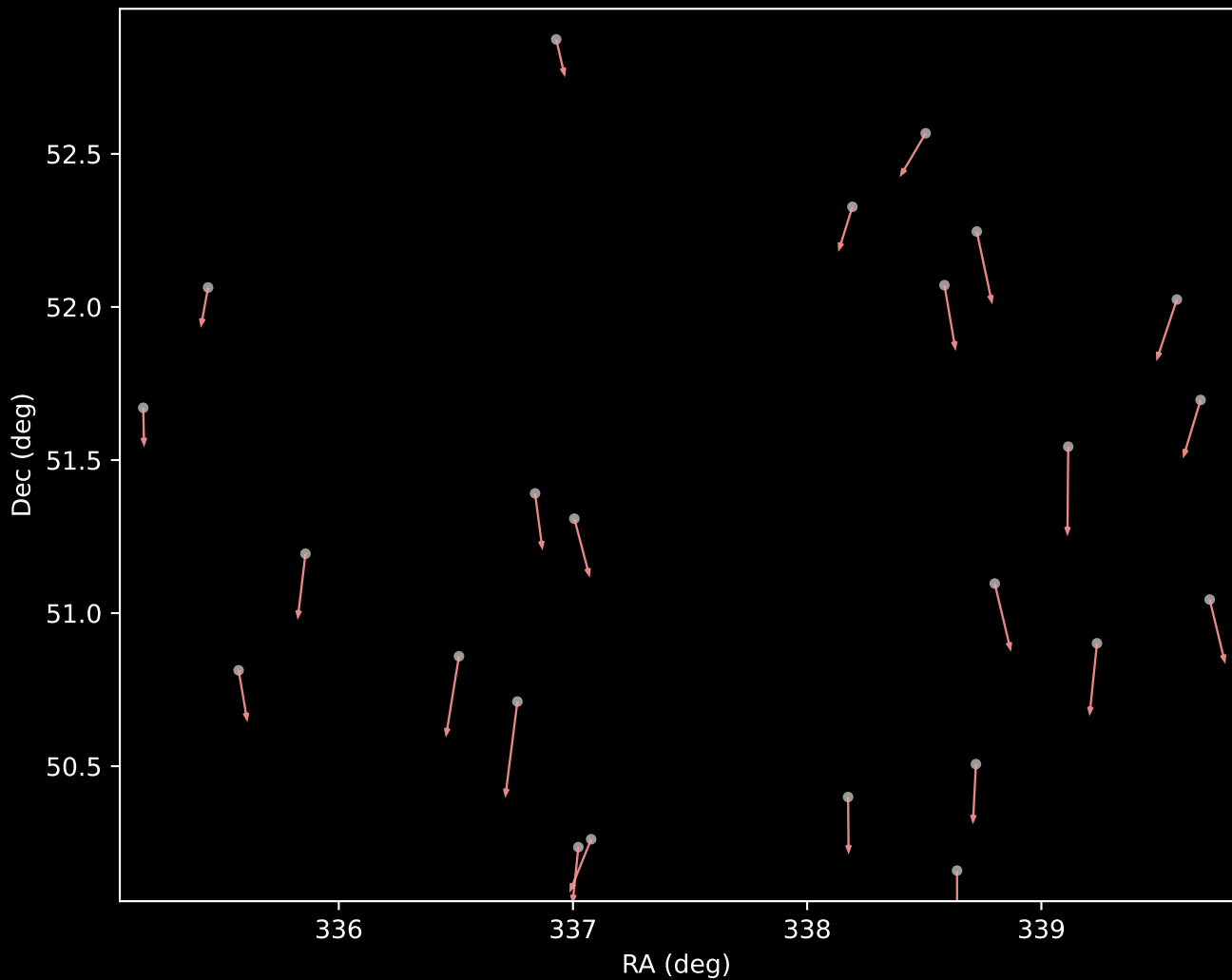
APOGEE DR17 Cluster 7 Proper Motion Vectors (n=24)
