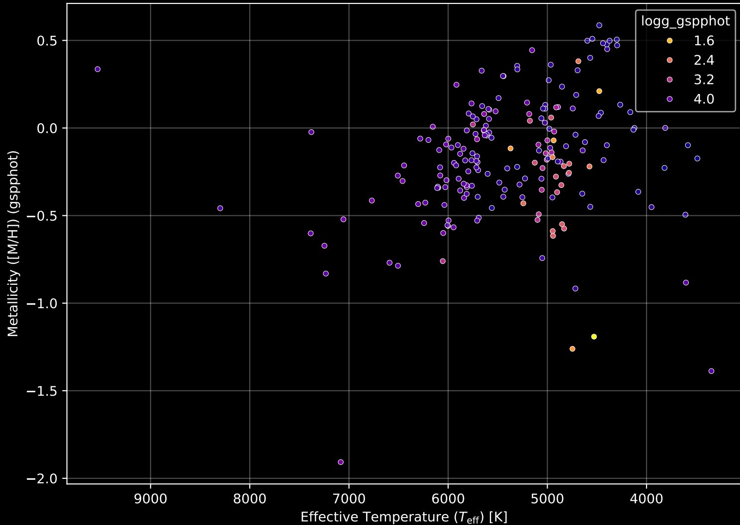
APOGEE DR17 Field: [081+49_MGA] Stellar Population Parameters (n= 195)
