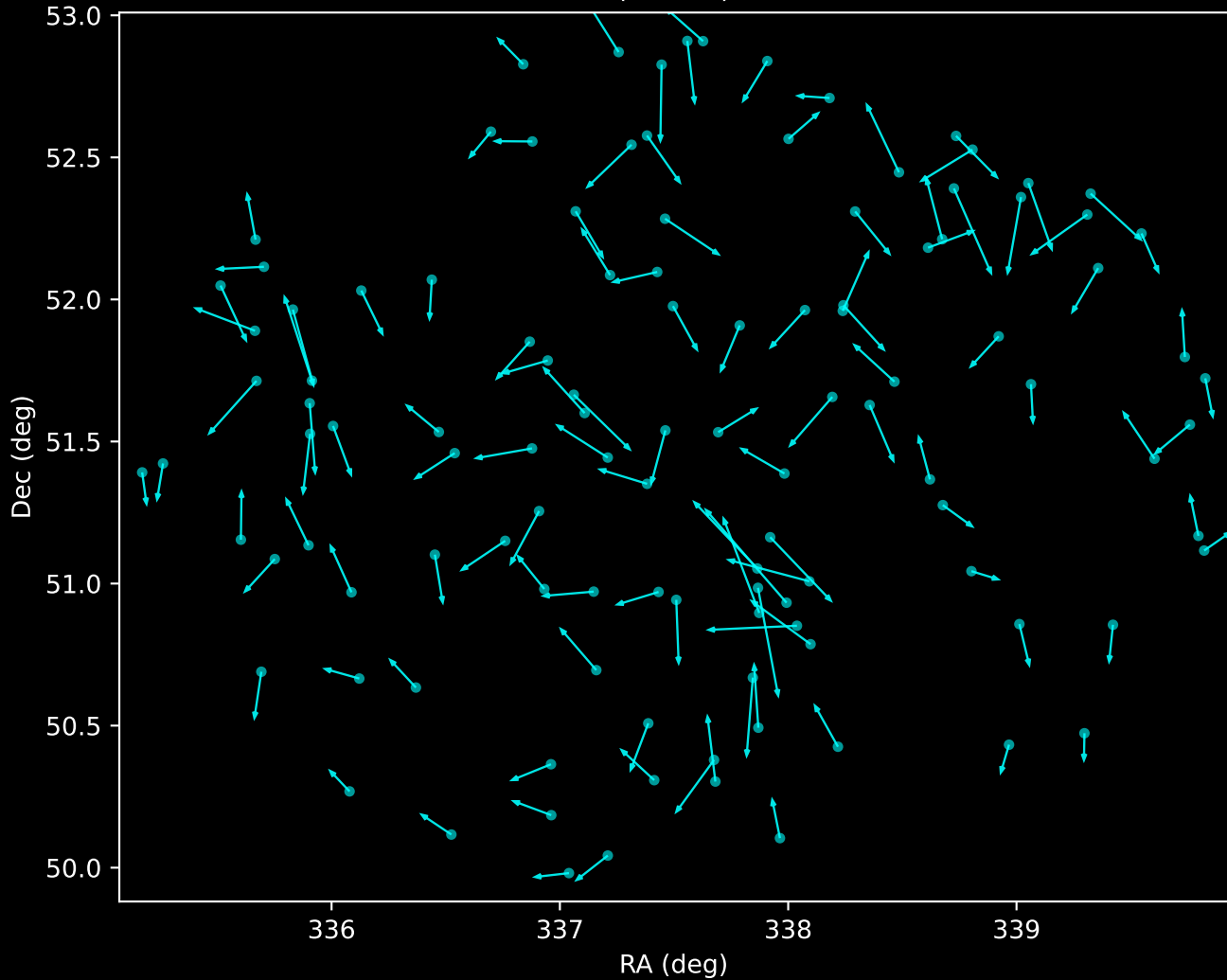
APOGEE DR17 Noise Stream Proper Motion Vectors (n=115)
